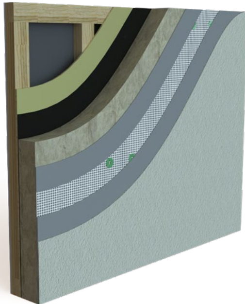
Typical Section through EWI System onto Timber
