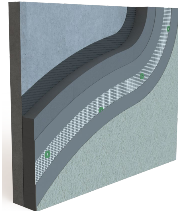
Typical Section through EWI System onto Masonry
