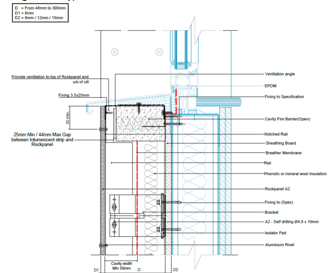
Diagram 8 - Typical window cill detail
