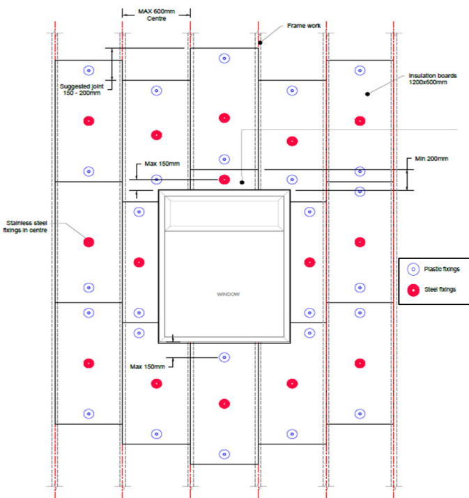
Diagram 3 - Typical insulation fixing pattern
