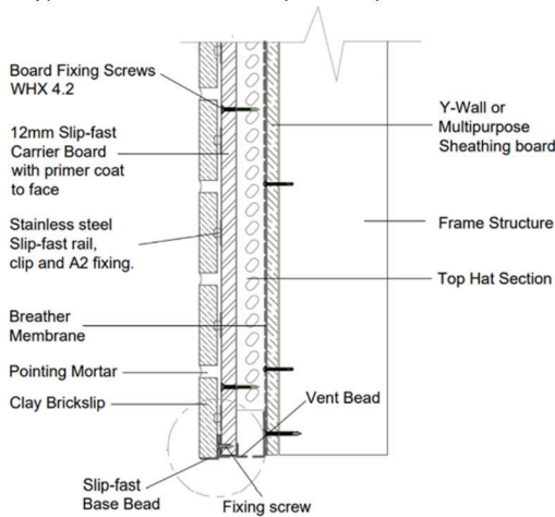
Diagram 2 - typical starter track with Slip Fast Top Hat Rail
