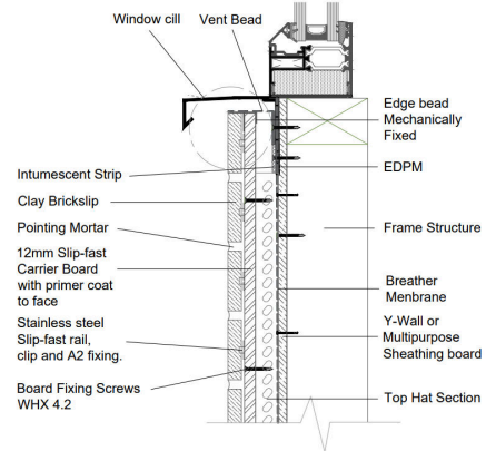
Diagram 7 - typical cill with Slip Fast Top Hat Rail
