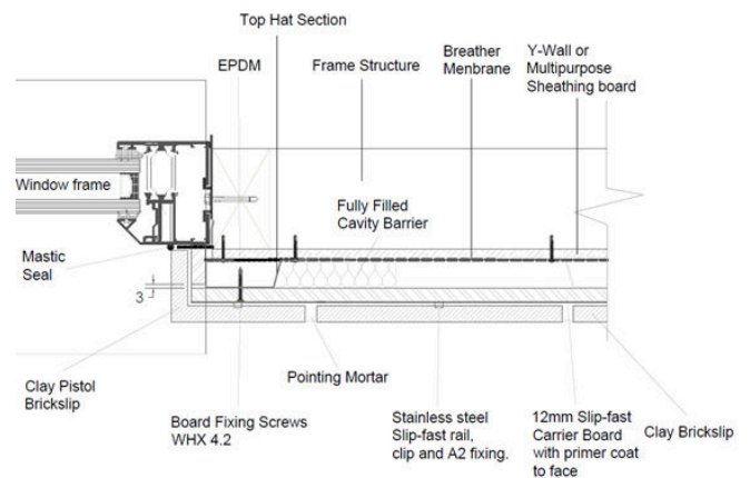
Diagram 3 - typical window jamb with Slip Fast Top Hat Rail
