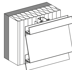
RIVETED WEATHER BOARDING on aluminium substructure
