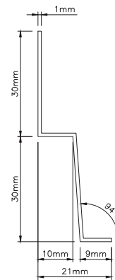
STARTER PROFILE Used to commence a run of Supertech plank 3000mm long.
