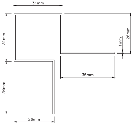
EXTERNAL CORNER (Symetrical) Used to provide protection of Supertech plank at external corners 3000mm long.
