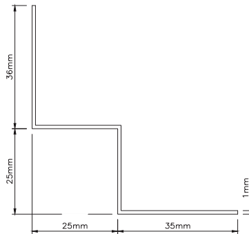
INTERNAL CORNER Used to provide a junction at Supertech plank Internal corners 3000mm long.
