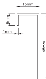
CONNECTION PROFILE End trim to terminate Supertech plank into a window reveal or soffit 3000mm long.
