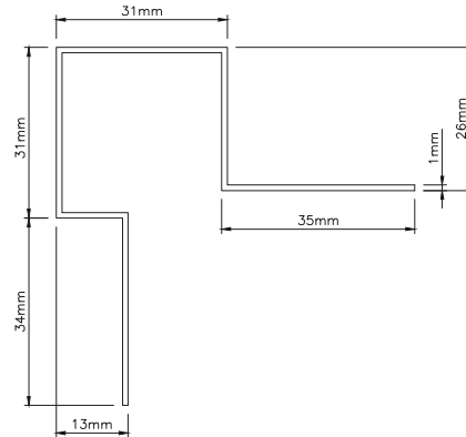
EXTERNAL CORNER/WINDOW REVEAL (Asymetrical) Used to provide protection of Supertech plank at corners into window reveals 3000mm long.
