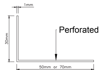
PERFORATED PROFILE Designed to allow air to flow through the system whilst protecting against vermin and some insects 3000mm long.
