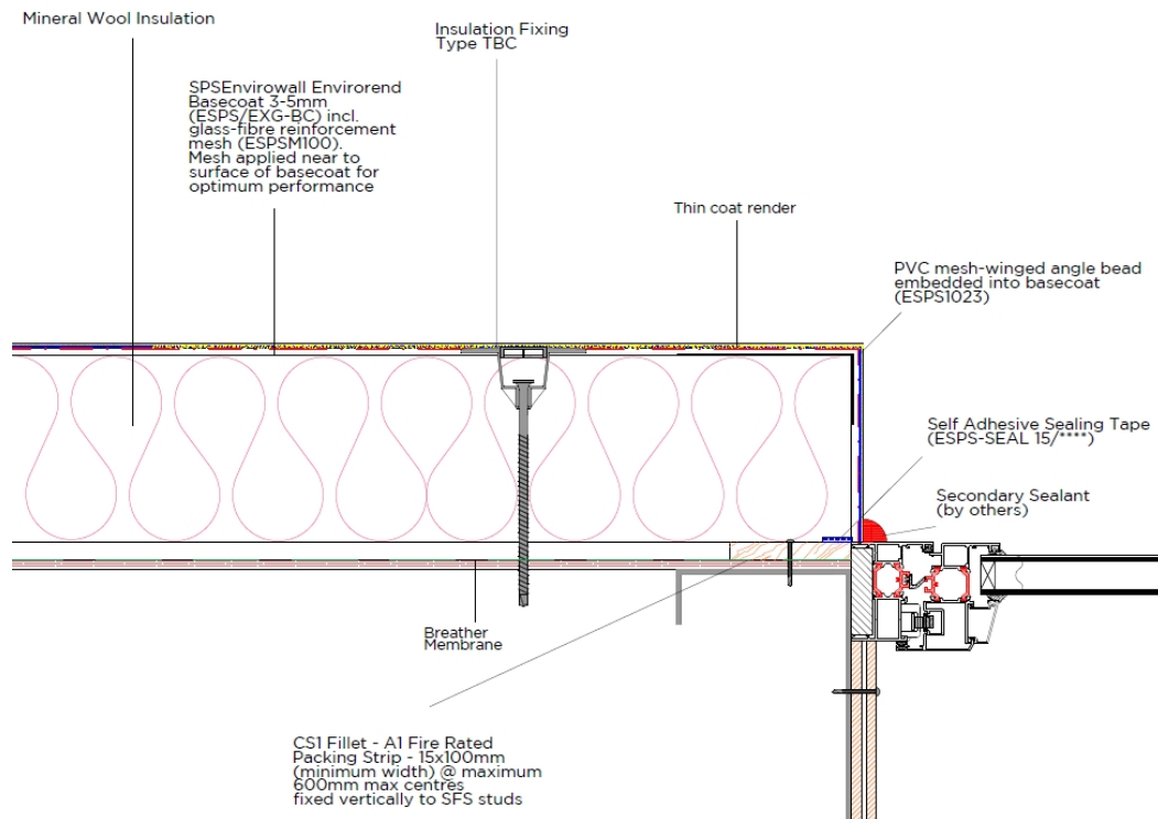
Figure 4 - Vertical firebreak detail
