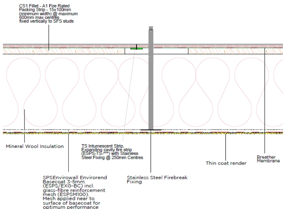
Figure 2 - Horizontal firebreak detail - plan view
