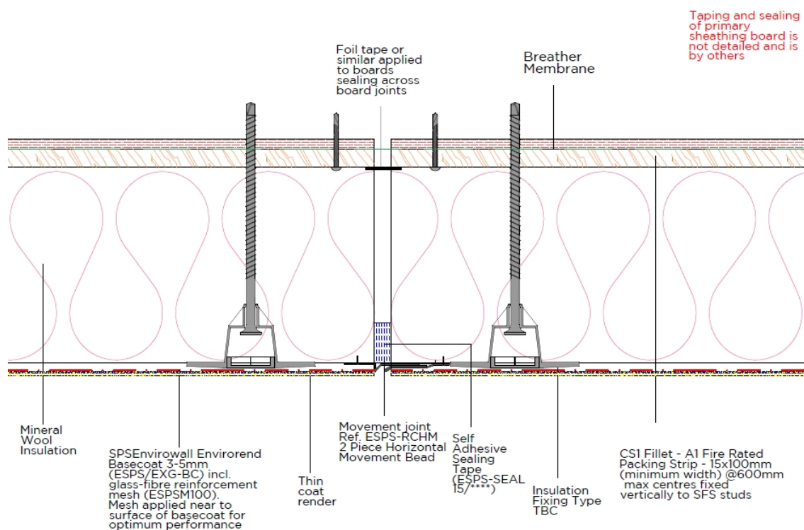
Figure 6 - Horizontal movement joint detail
