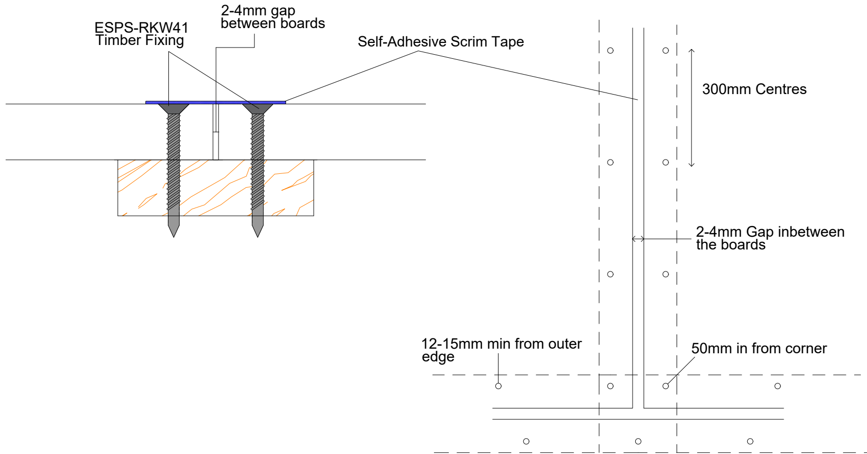
L Shaped Boards cut around Apertures
